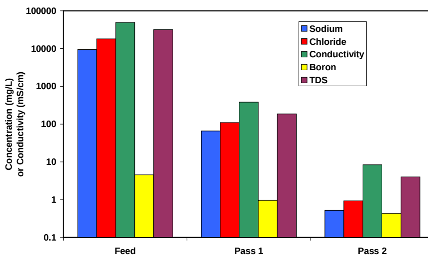
Figure 2. Levels of selected seawater components at various stages of the desalination process.
