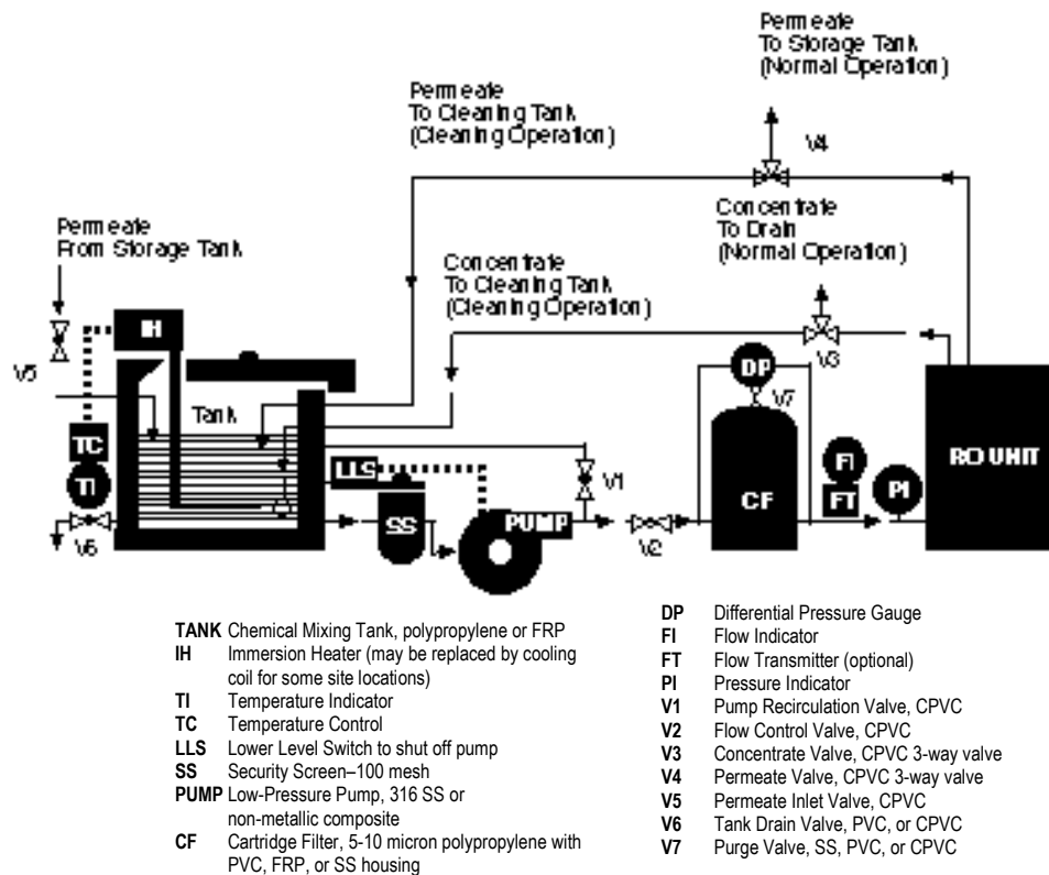
Figure 6.1 Cleaning system flow diagram
