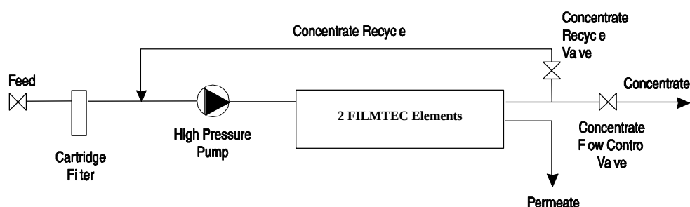
Figure 3.3 Single-module system
