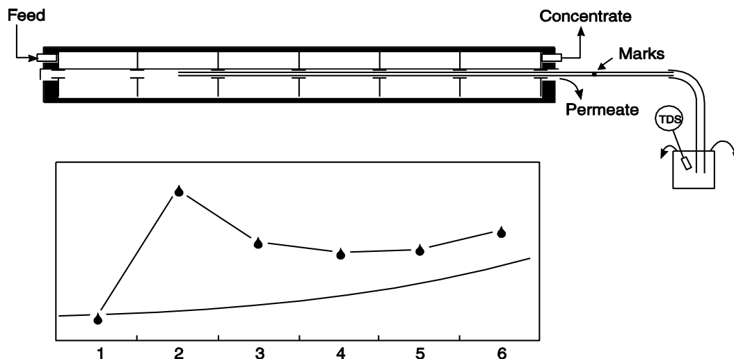
Figure 8.1 Conductivity profile
