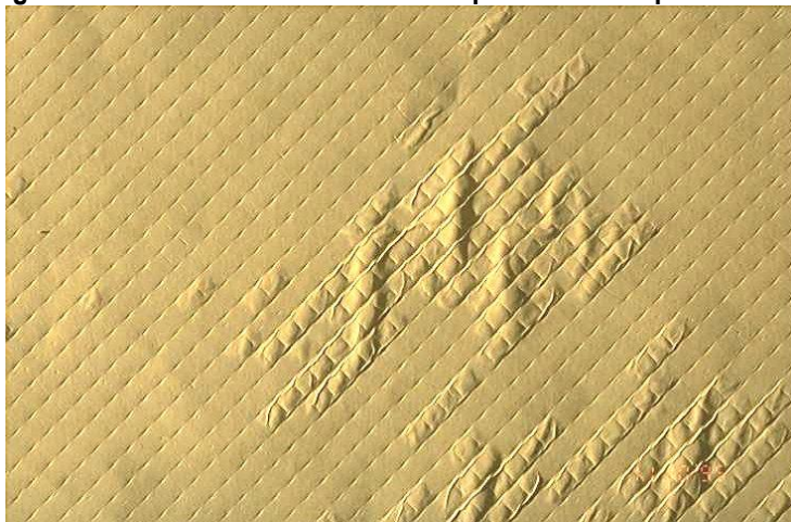
Figure 8.8 Picture of membrane with permeate backpressure damage
