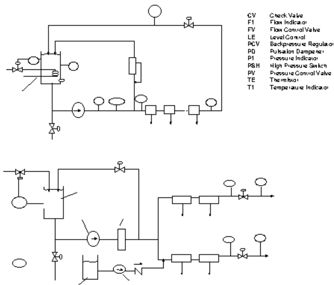
Figure 9.6 Flow schematic
