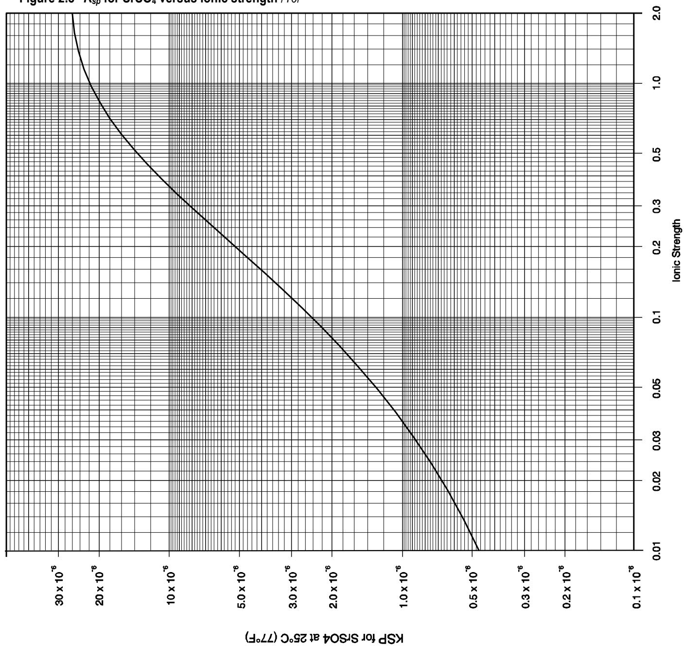
Figure 2.8 K_{sp} for \text{SrSO}_4 versus ionic strength I
