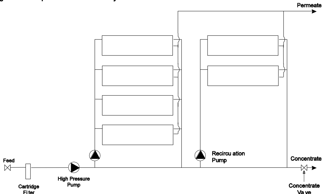
Figure 3.8 Tapered recirculation system
