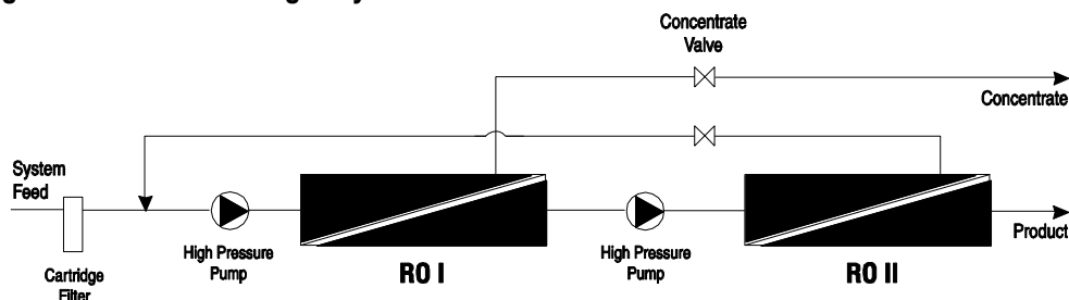
Figure 3.9 Permeate staged system
