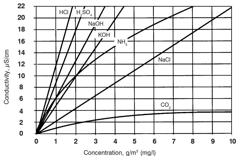
Figure 9.2 Conductivity of ionic solutions at 77°F (25°C)
