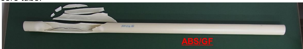
Permeate core tube collapse and mechanical failure.
