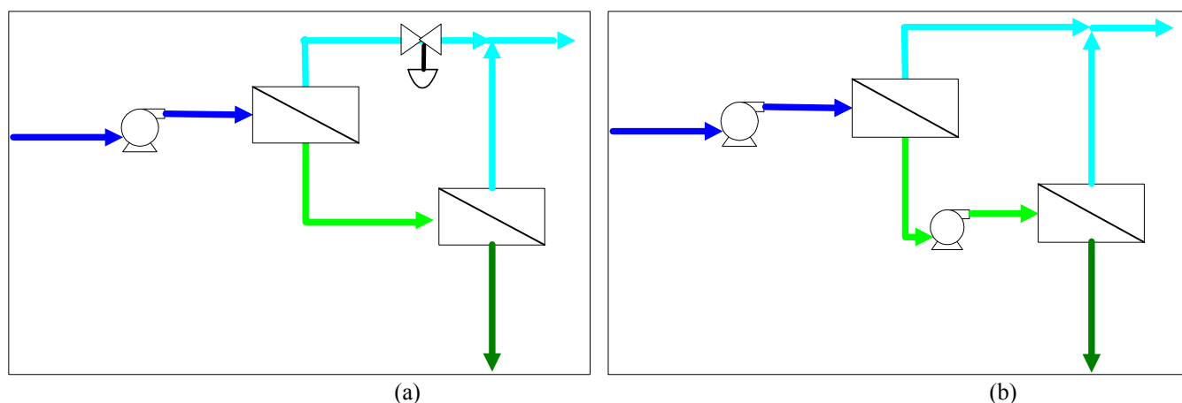
Two Stage RO System with (a) Permeate Throttling Valve After First Stage (b) Booster Pump Before Last Stage.
