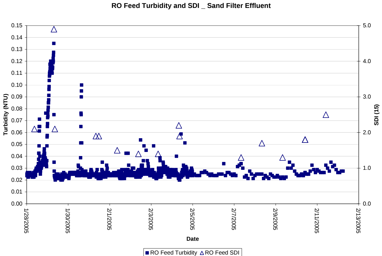
Figure 8. Sand filter filtrate water quality (turbidity and SDI) during wet weather conditions.
