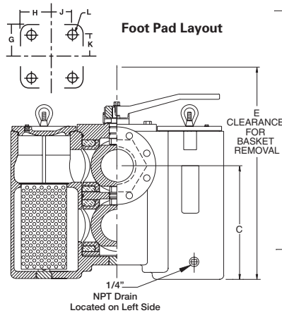
Front View Flanged and Threaded Models
