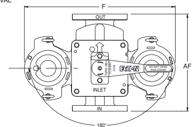
Top View Flanged Model
