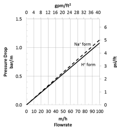
Figure 2: Pressure Drop
