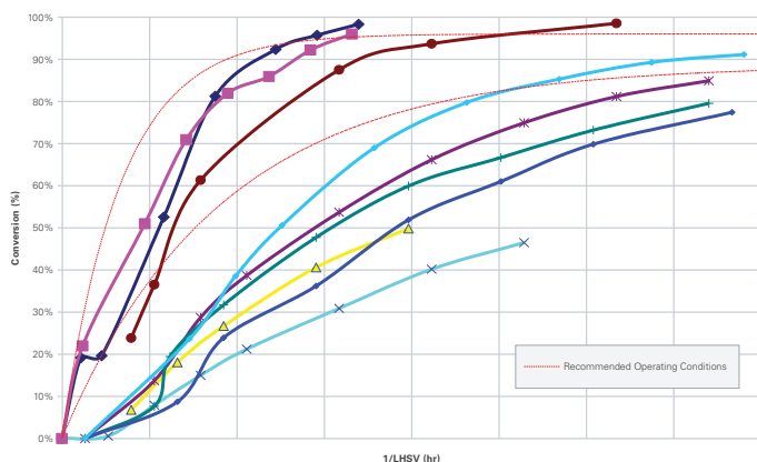
Figure 2: Conversion Profile of Esterification Reaction Data using Dow's Amberlyst BD20
