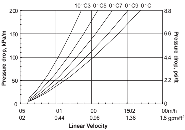
Figure 2. Pressure Drop
