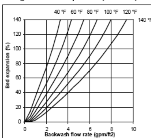
Figure 4 Bed Expansion (US units)
