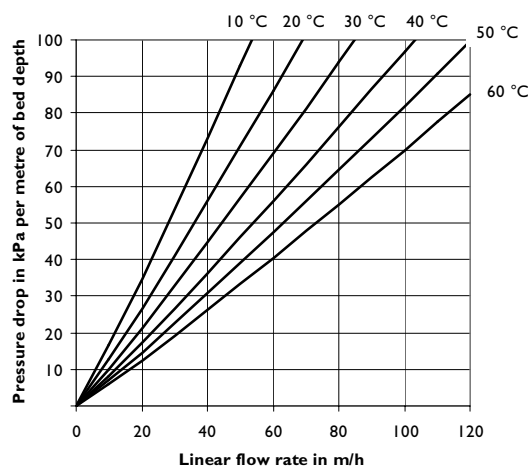
Fig. 2 : Pressure Drop
