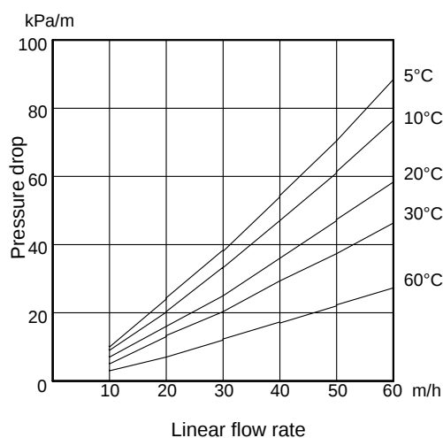
Fig. 2 : Pressure Drop
