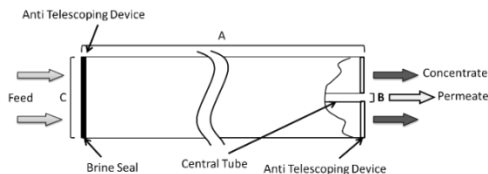
Figure 1: Element Dimensions Diagram, Female 8040
