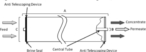
Figure 2: Element Dimensions Diagram, Male 2540 & 4040
