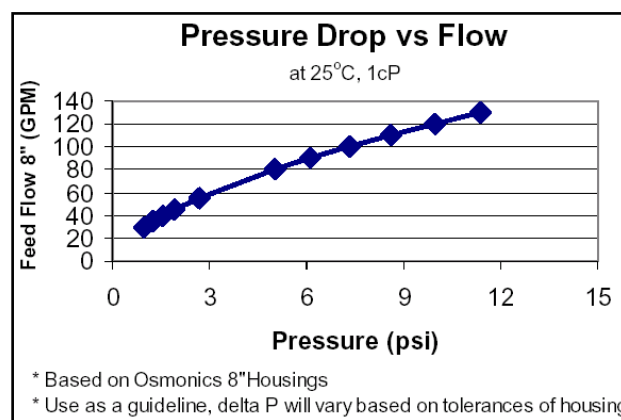
Figure 7: Pressure Drop for 8" Element
