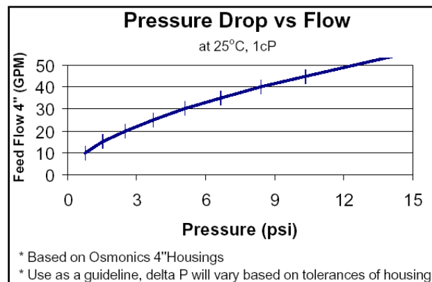
Figure 6: Pressure Drop for 4" Element
