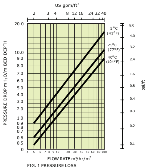
FIG. 1 PRESSURE LOSS
