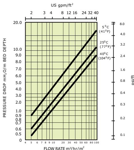
FIG. 1 PRESSURE LOSS
