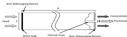
Figure 1 : Element Dimensions Diagram
