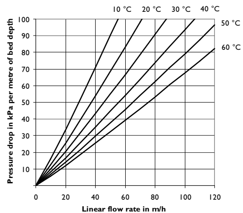
Fig. 2 : Pressure Drop
