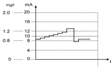
Example 1 measuring point, Interface 0-20 mA
