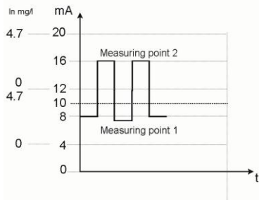
Example: 2 Measuring points, Interface 4 -20 mA
