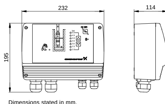
Fig. 19 Dimensional sketch of the CU 301
