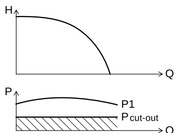
Fig. 2 Dry-running protection
