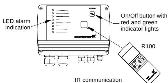
Fig. 21 Front view of the CU 300
