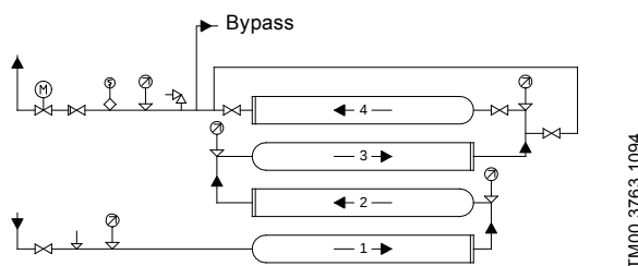
Fig. 10 Booster unit with four modules connected in series with bypass, mounted above each other
