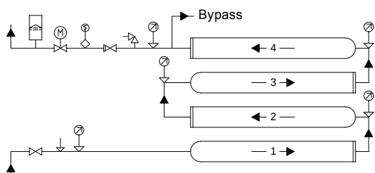
Fig. 7 Booster unit with four modules connected in series, mounted above each other
