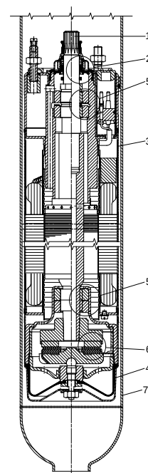
Fig. 6 Example, MS 4000
