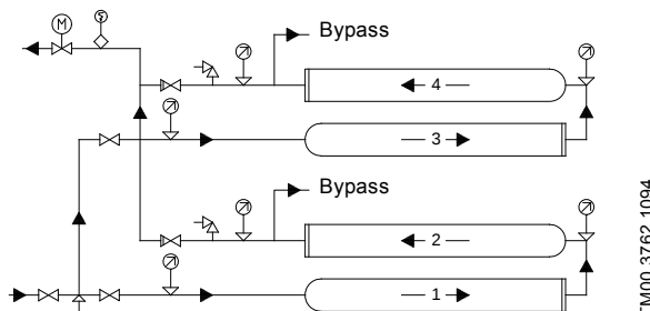
Fig. 9 Booster unit with two modules connected in series and in parallel, mounted above each other
