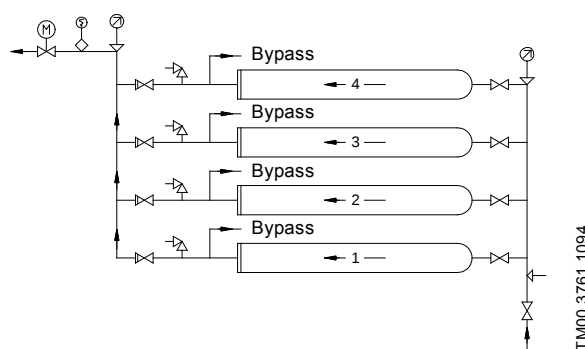
Fig. 8 Booster unit with four modules connected in parallel, mounted above each other
