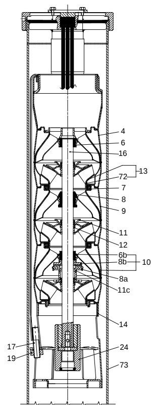
Fig. 5 Example, BM 46
