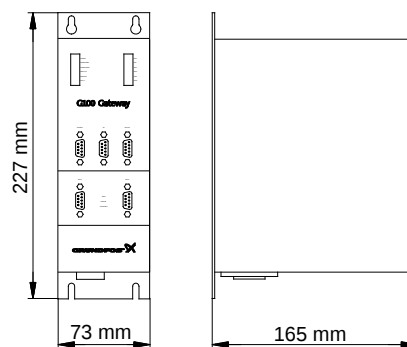
Fig. 18 Dimensional sketch
