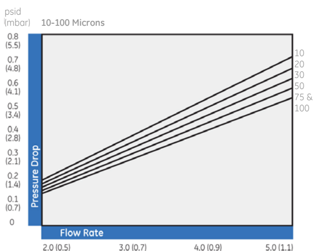
Figure 3: High Flow Rate at Low Pressure Drop 1
