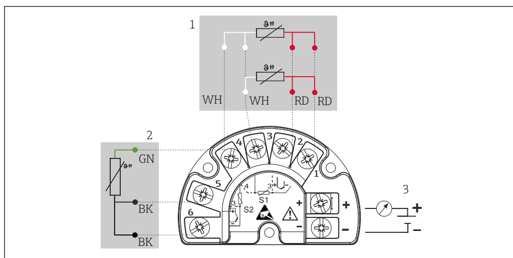
6 Field mounted transmitter TMT162 (dual input)
