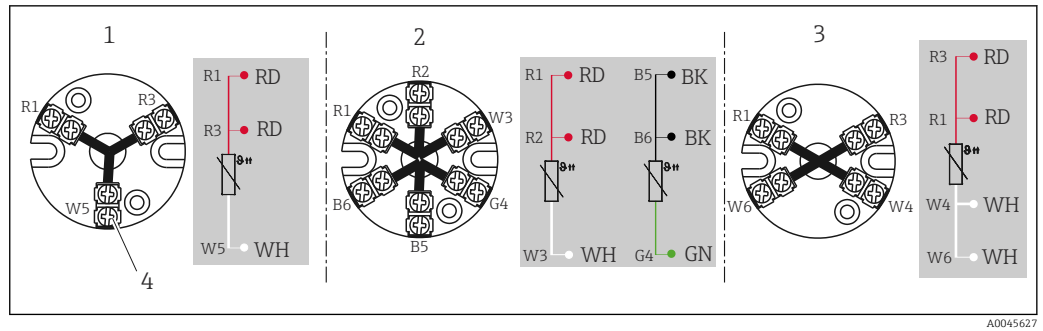
8 Terminal block mounted
