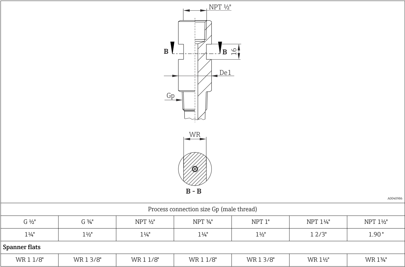
De1 size matrix for screw-in thermowells in mm (in)
