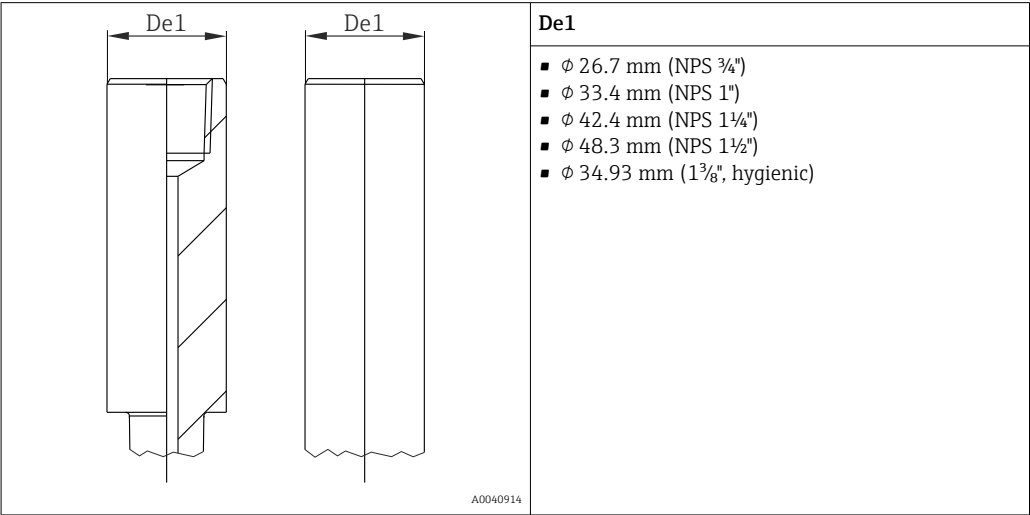
Weld-in version/socket weld
