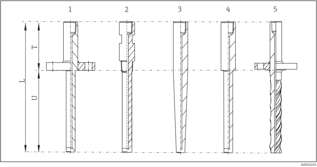
2 Typical ASME design, iTHERM TwistWell and references
