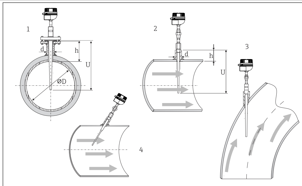
14 Installation examples
