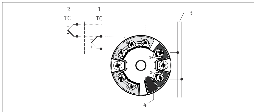
10 Head-mounted transmitter TMT8x (dual sensor input)
