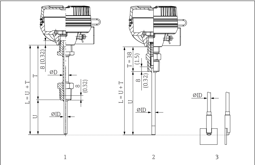
Thermometer with fixed process connection
