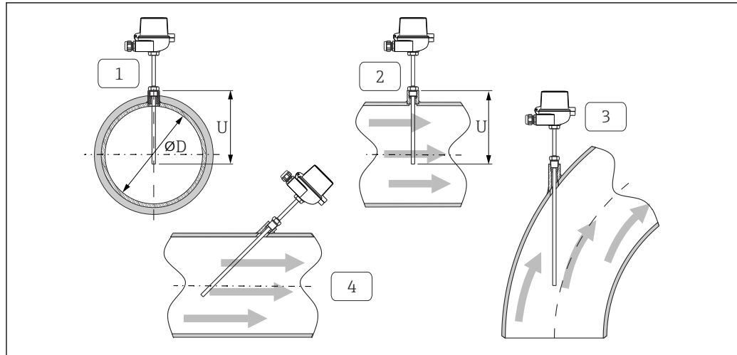
13 Installation examples
