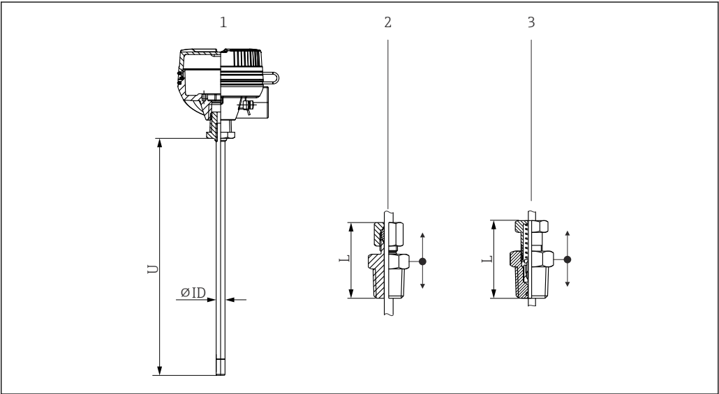
Thermometer without fixed process connection
