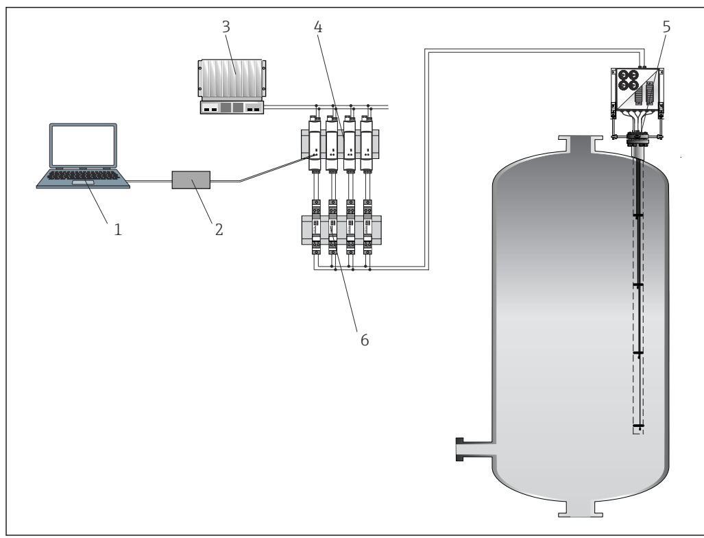
1 Application example in a reactor, mounted multipoint thermometer in a thermowell available on site with four measurement points and four built-in transmitters or terminal blocks.
