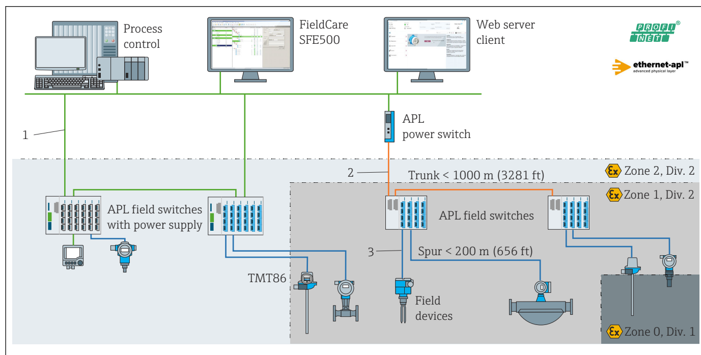
2 Equipment architecture of the transmitter with PROFINET with Ethernet-APL communication
