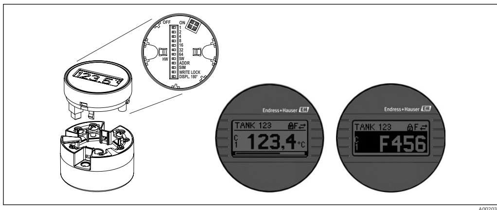
7 Attachable measured value display TID10 with bar graph indicator (optional)
