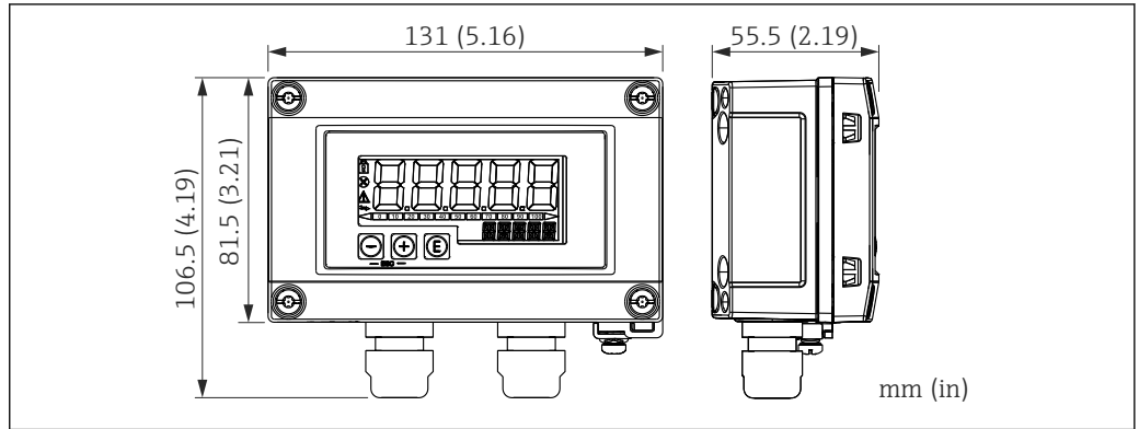
5 Dimensions of RIA15 in field housing, engineering unit: mm (in)
