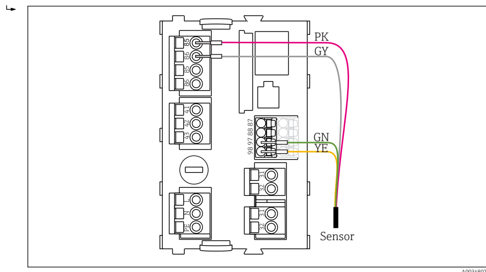
3 Sensor connection
