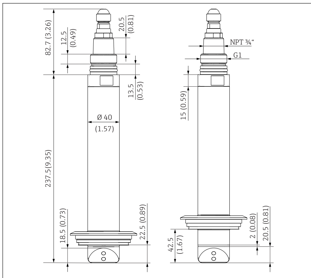
24 Dimensions of stainless steel sensor with standard Varivent connection (left) and extended shaft (right). Dimensions: mm (in)
