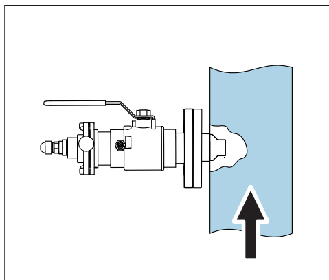
16 Installing with CUA451 retractable assembly
