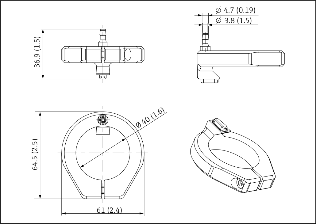
20 Dimensions for compressed air cleaning. Dimensions: mm (in)
