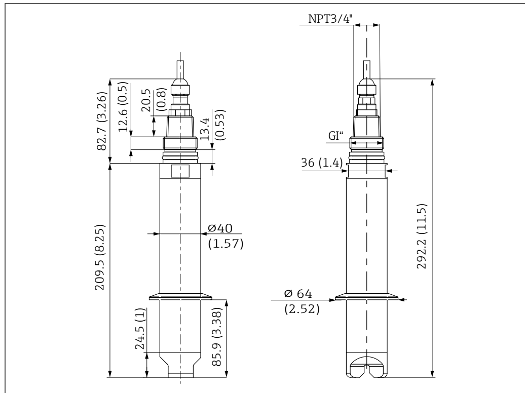
19 Dimensions with clamp. Dimensions: mm (in)
