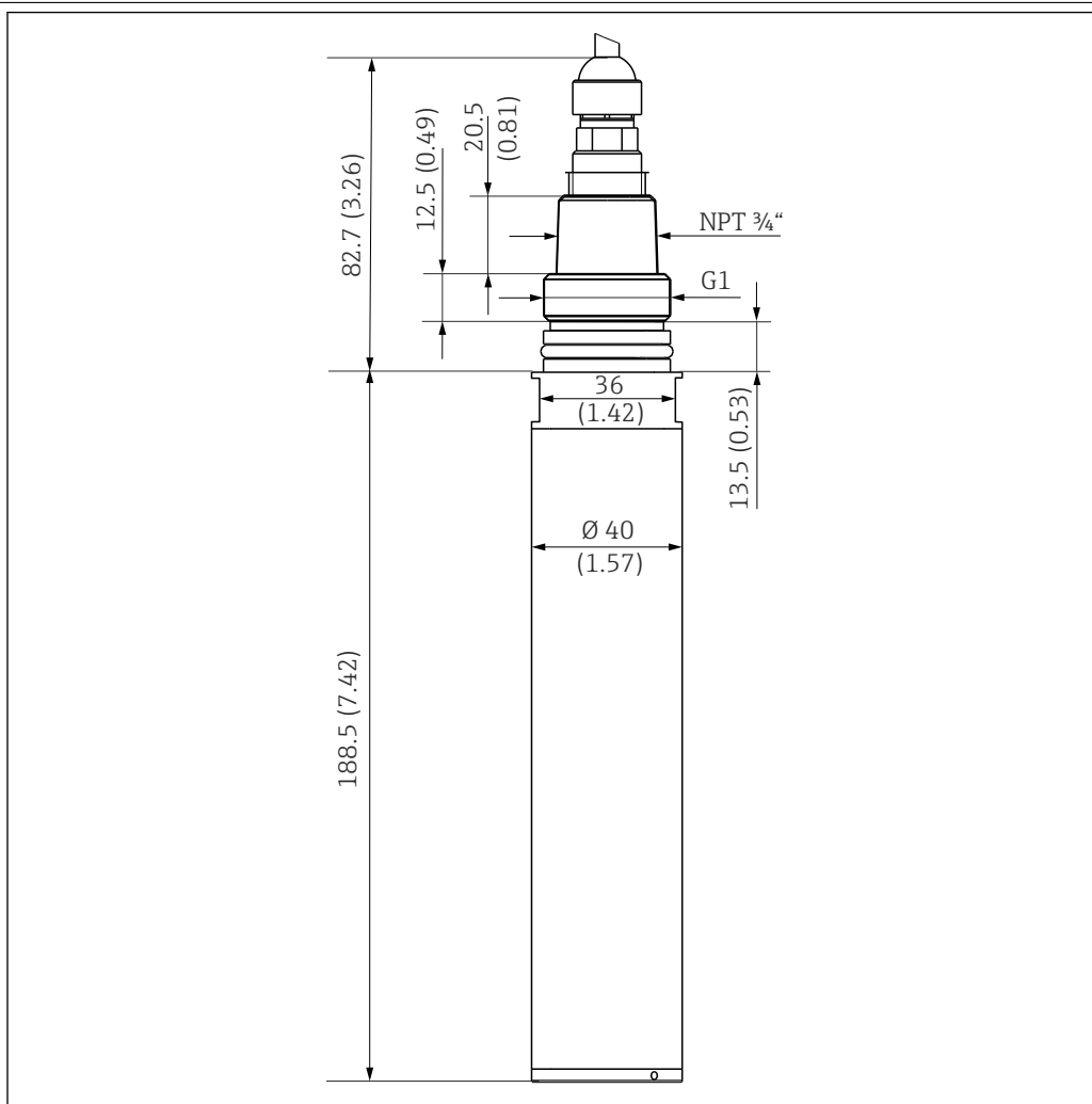
21 Dimensions. Engineering unit: mm (in)
