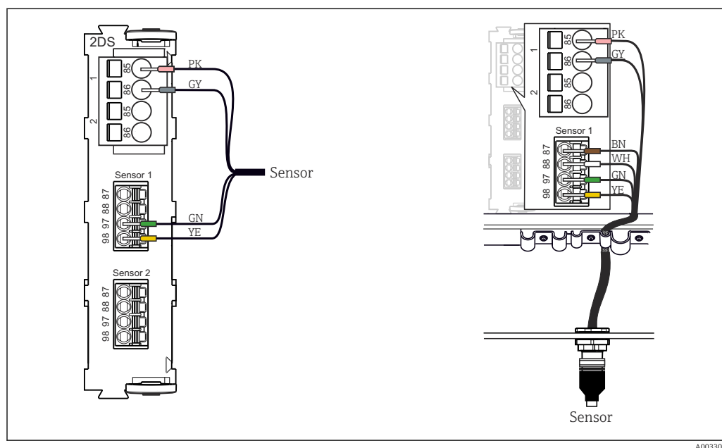
13 Sensor connection to sensor input (left) or via M12 plug (right)
