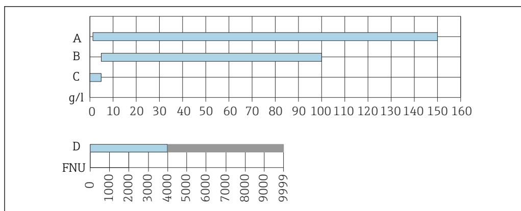
14 Clear water application type
