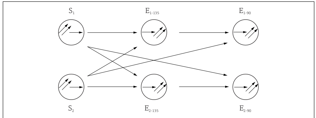
5 4-beam pulsed light method
