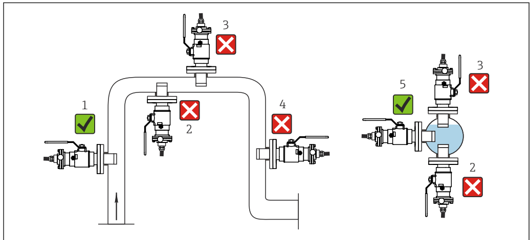
20 Orientations and positions (with CUA451 retractable assembly)
