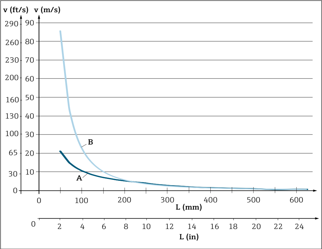
9 Permitted flow velocity, thermowell diameter 9 mm (0.35 in) A Medium water at T = 50\text{ °C} (122 °F) B Medium superheated steam at T = 160\text{ °C} (320 °F) L Immersion length exposed to flow v Flow velocity
