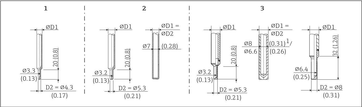
12 Thermowell tips available (reduced, straight or tapered)
