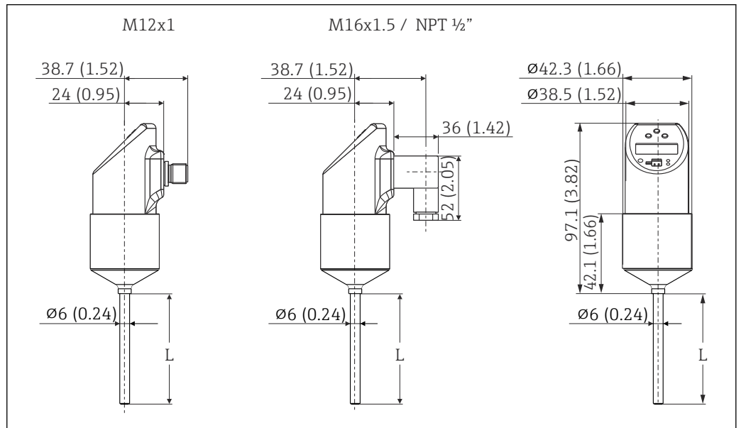
7 All dimensions in mm (in)
