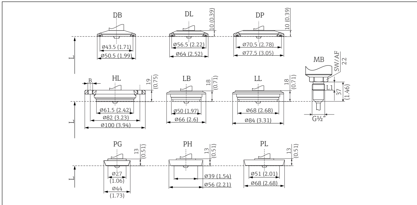
9 Process connection versions, all dimensions in mm (in).
