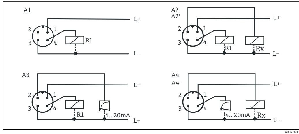
2 Thermophant T TTR3x with M12x1 connector
