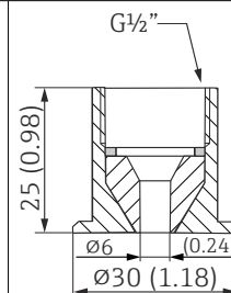
13 Dimensions in mm (in)
