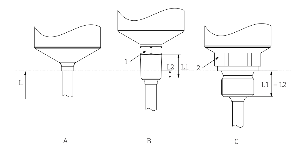
8 Process connection versions
