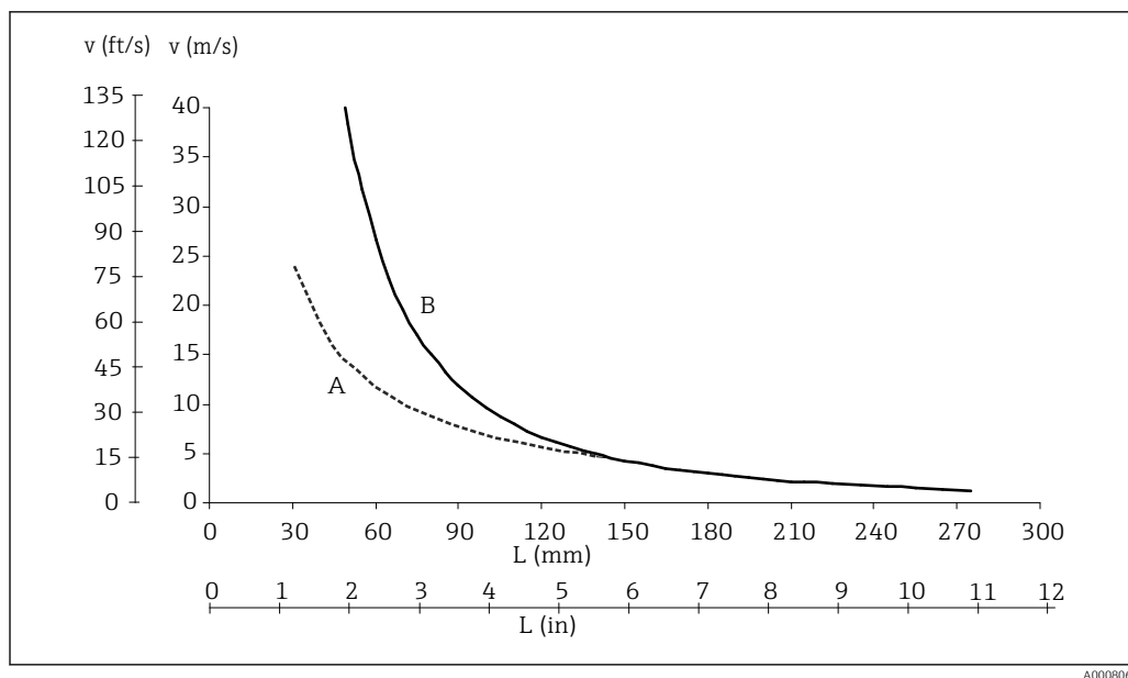
6 Permitted flow velocity
