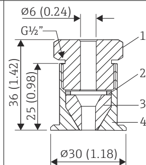
12 Dimensions in mm (in)
