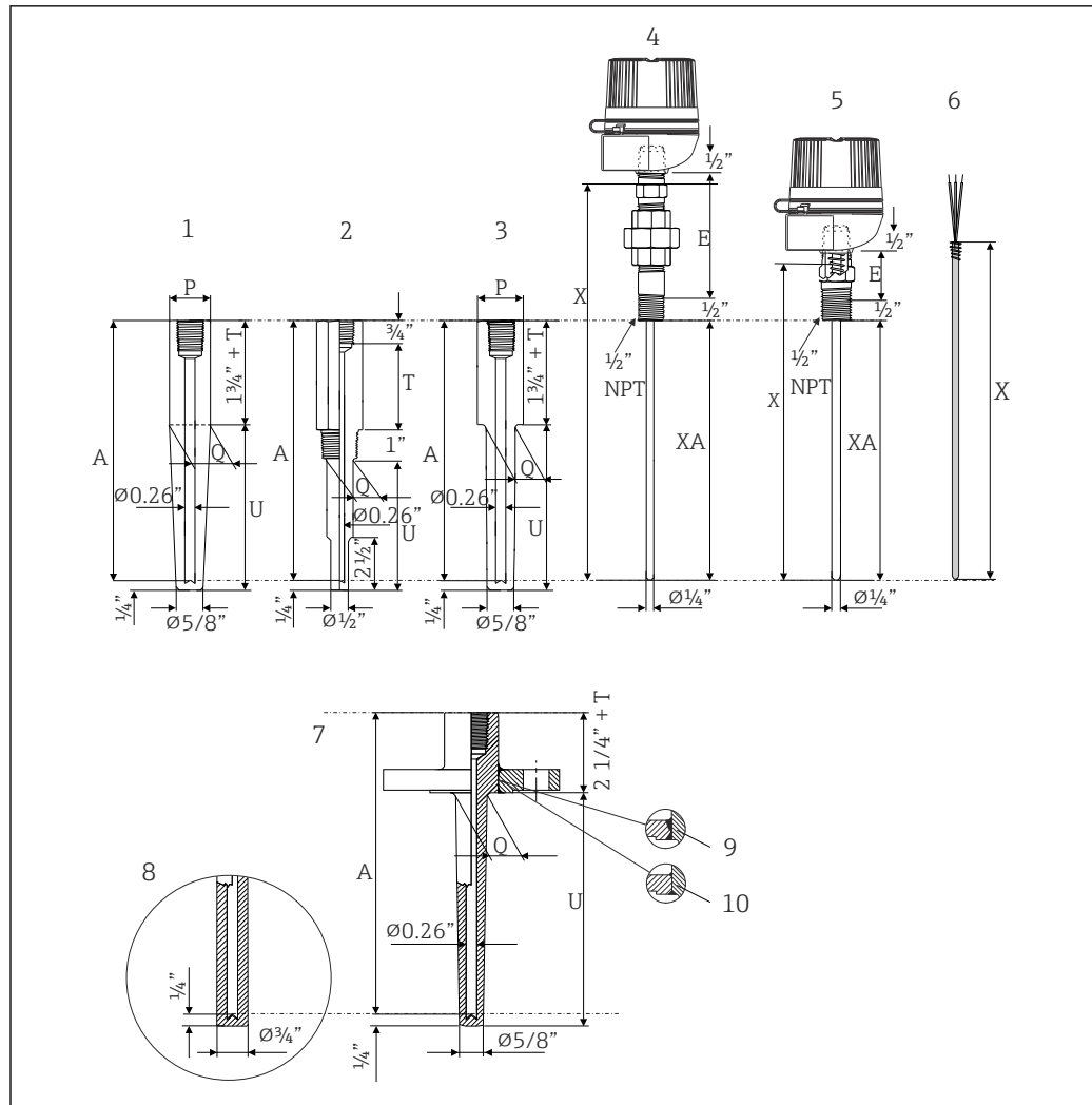
8 Dimensions of the sensor assemblies.
