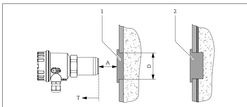
13 Mounting in front of microwave-impermeable process wall
