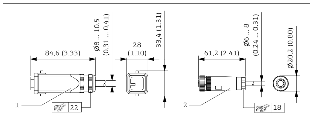
27 Mating connectors. Unit of measurement mm (in)
