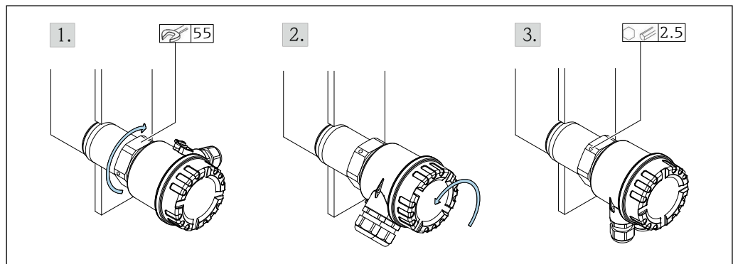
■ 12 Mounting with connection thread
