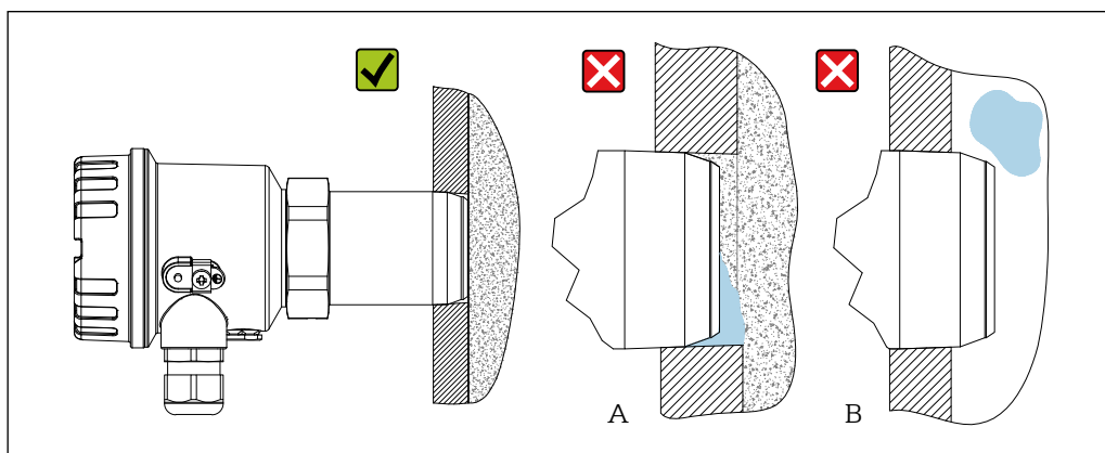
10 Direct mounting with threaded connection
