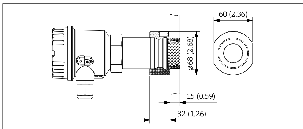
35 Dimensions high pressure adapter. Unit of measurement mm (in)
