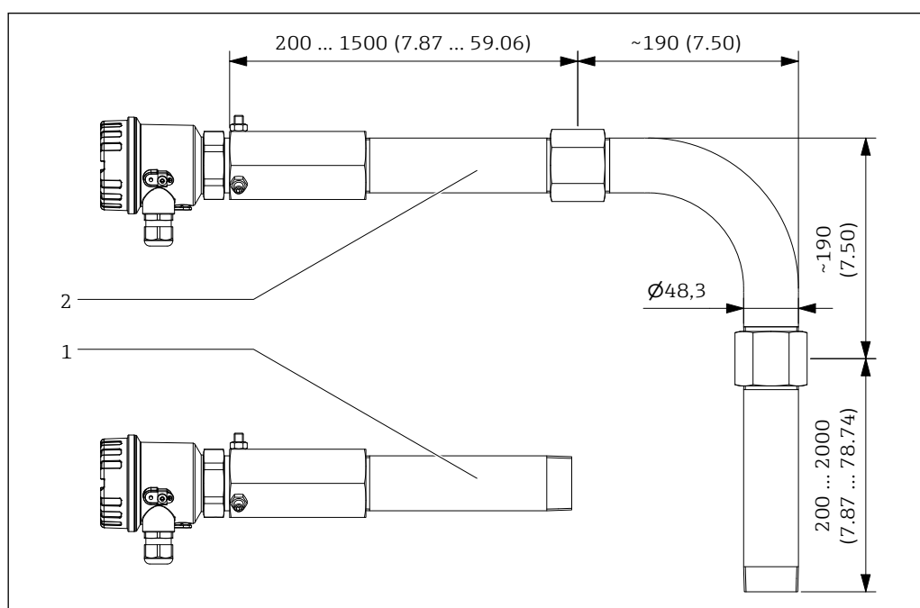
42 Dimensions wave guide. Unit of measurement mm (in)
