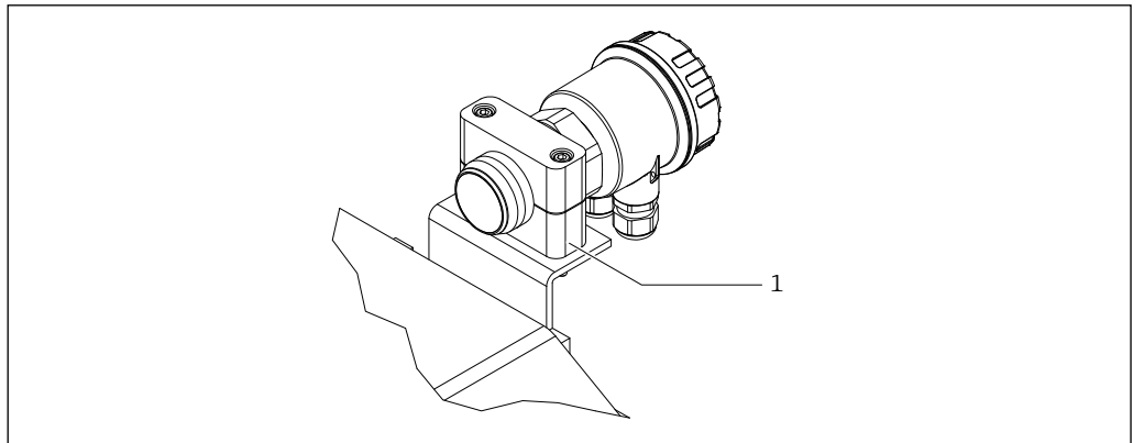
24 Mounting for open processes
