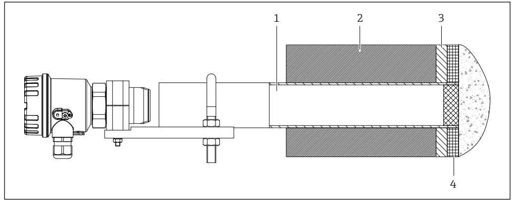
23 Mounting with spacer tube (wave guide)
