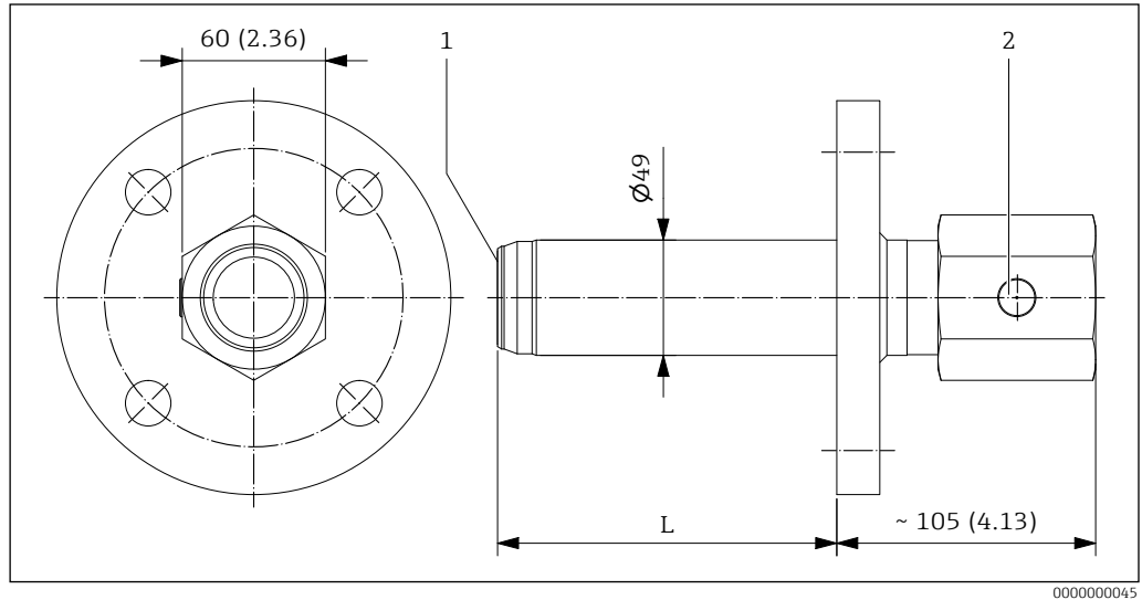
39 Dimensions insertion adapter. Unit of measurement mm (in)
