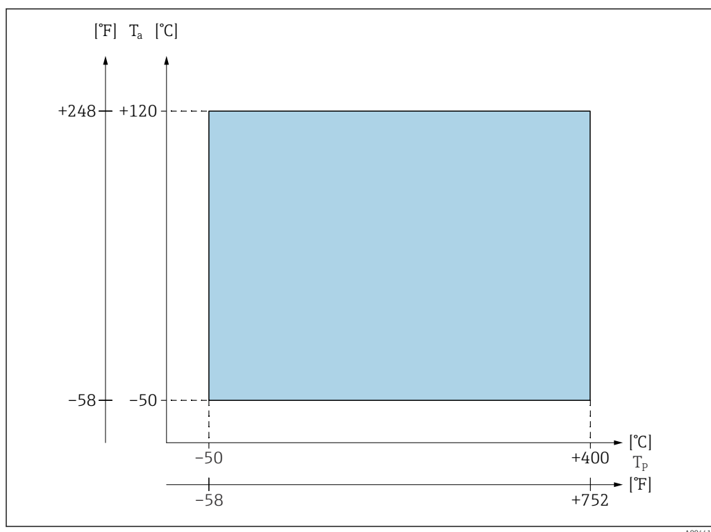
27 Process temperature diagram: separate housing
