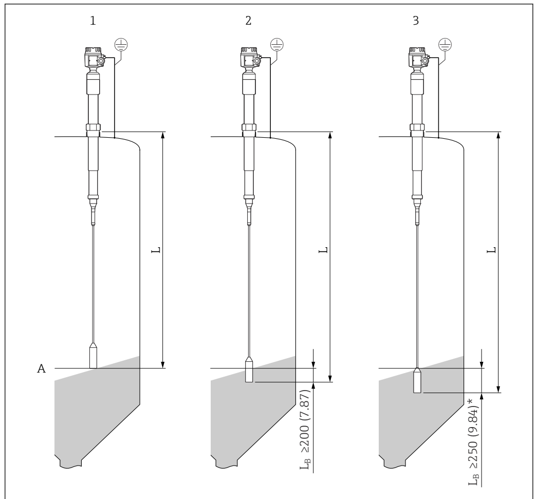
22 Rope length in correlation with the material. Unit of measurement mm (in)
