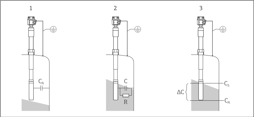
1 Measuring principle of capacitance point level detection
