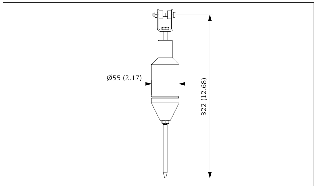
■ 20 Sensing weight for interface measurement in liquids with a significant difference in density. Unit of measurement mm (in)
