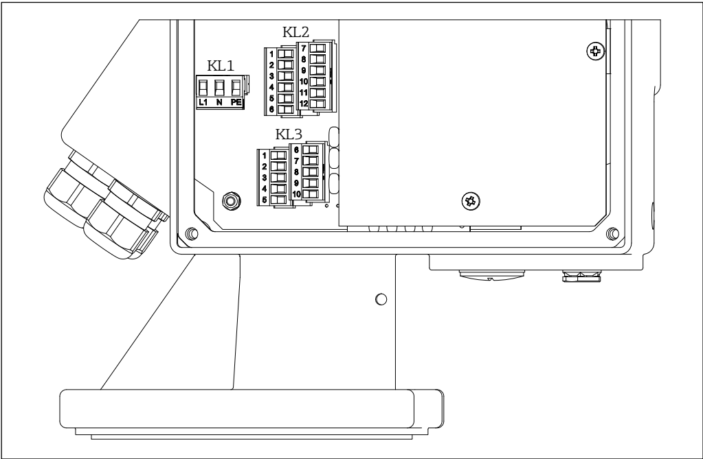
4 Terminal assignment
