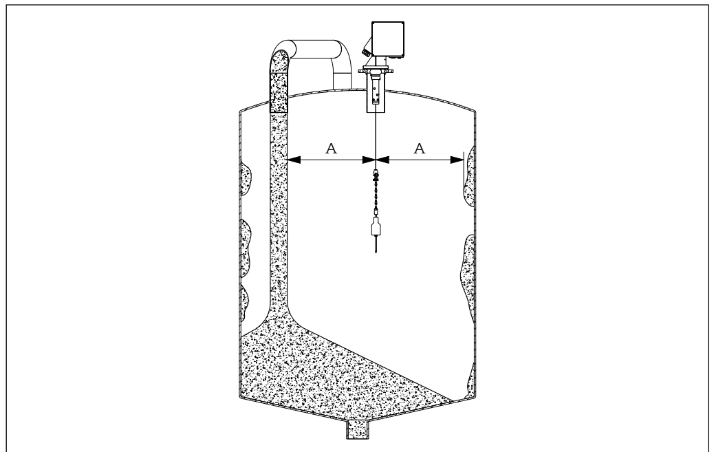
6 Installation position
