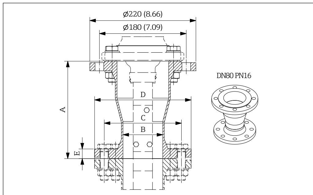
18 Process adapter (example DN80 PN16). Unit of measurement mm (in)
