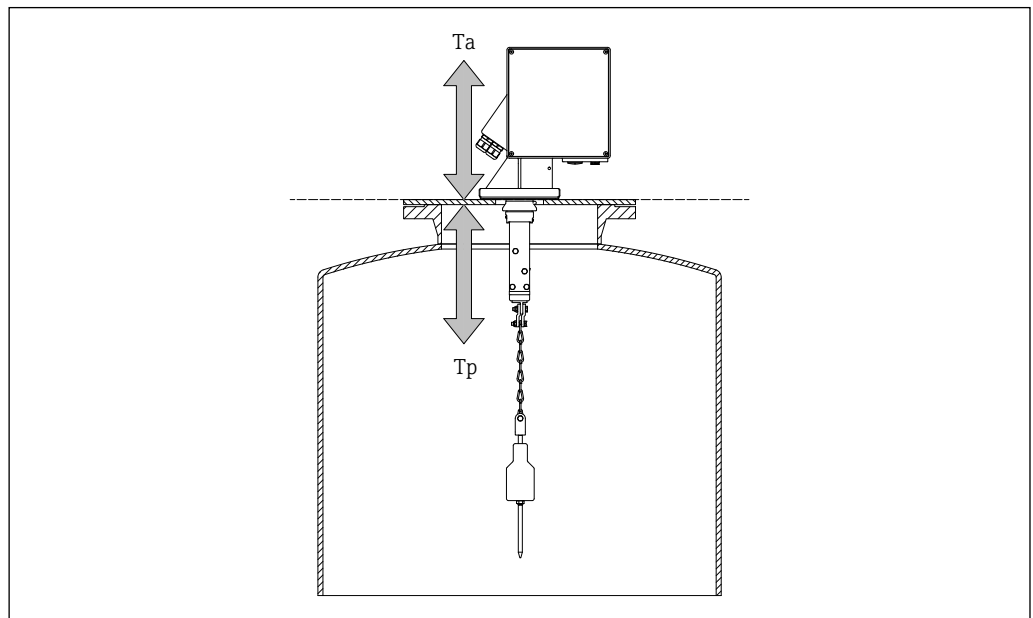
8 Permissible ambient temperatures at the FMM20
