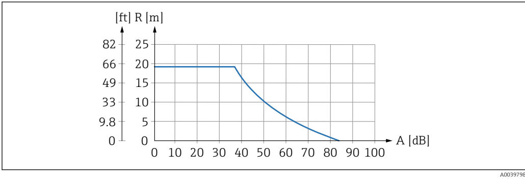
2 Range chart for ultrasonic sensors
