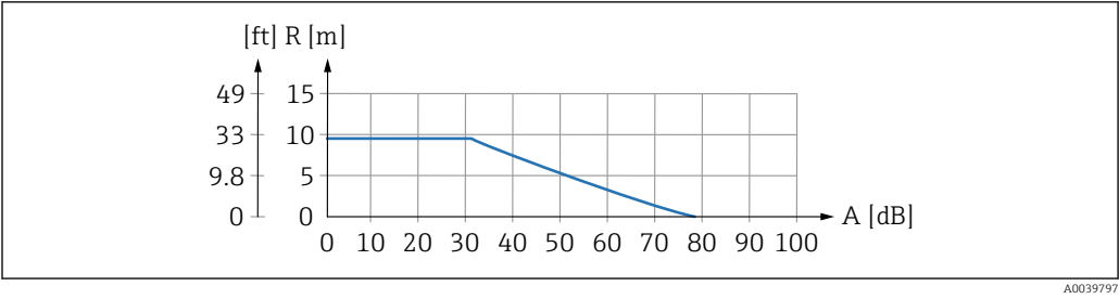
2 Range chart for ultrasonic sensors
