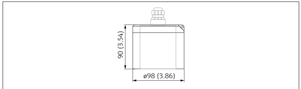
13 Weather protection cover. Unit of measurement mm (in)
