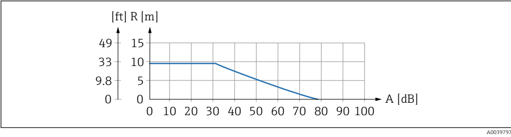
2 Range chart for ultrasonic sensors A Total attenuation in dB R Range in m (ft)
