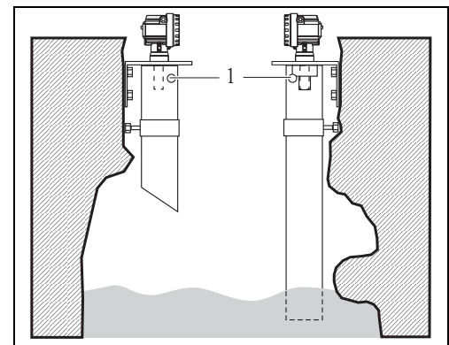
1 Venting hole
