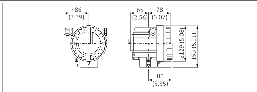
16 Dimensions of F12 housing. Unit of measurement mm (in)
