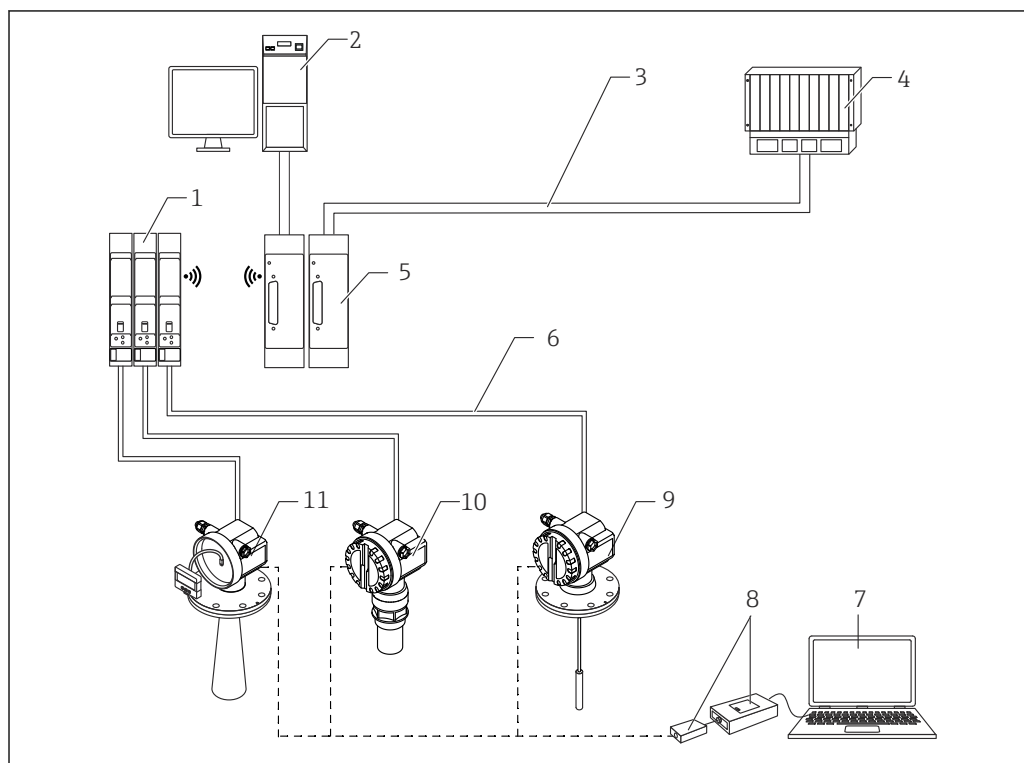
25 System integration via Endress+Hauser Rackbus
