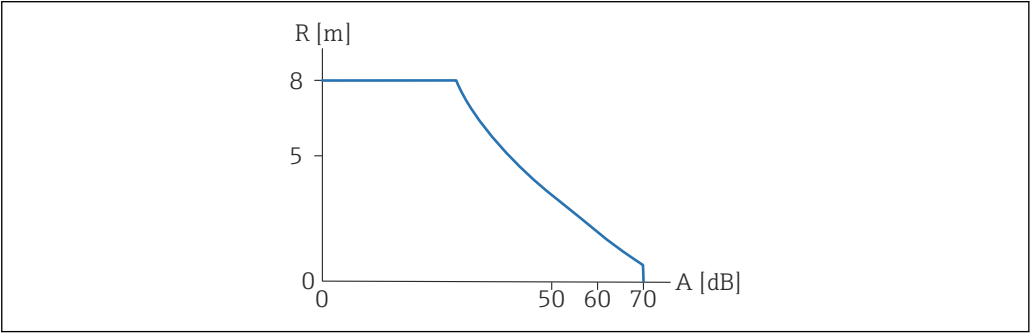
4 Range chart
