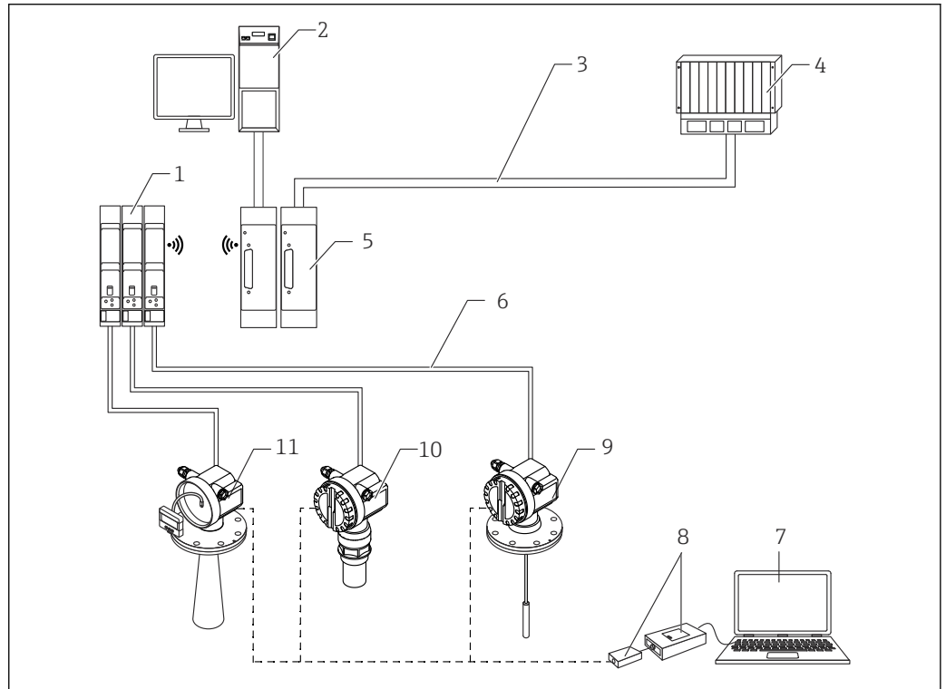
22 System integration via Endress+Hauser Rackbus
