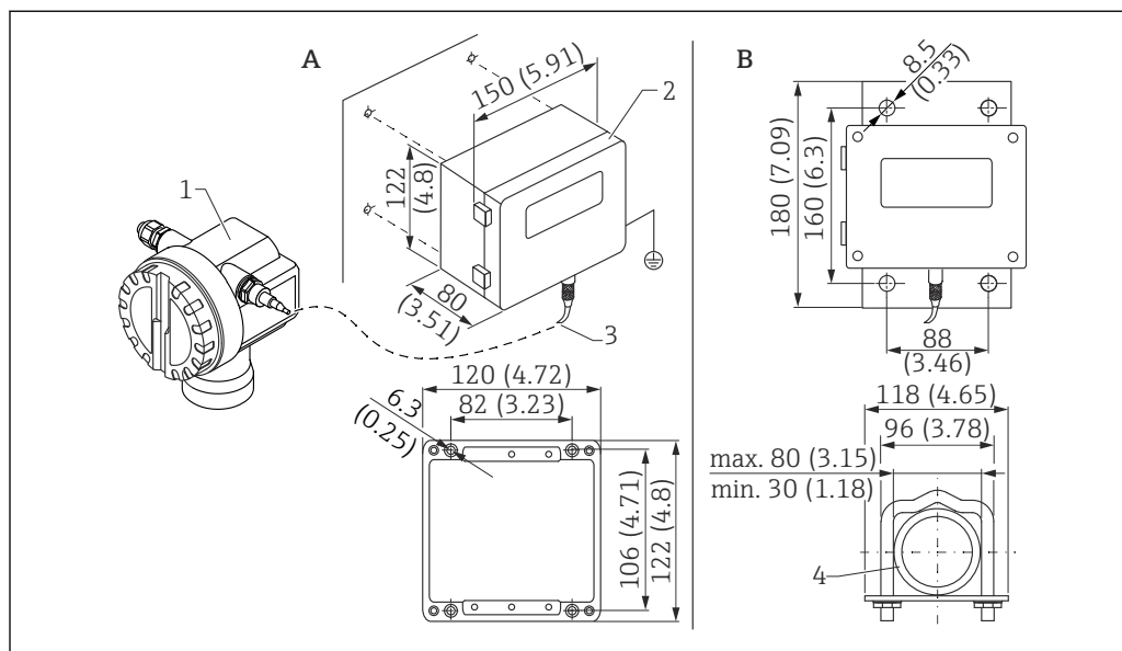
35 Remote display. Unit of measurement mm (in)
