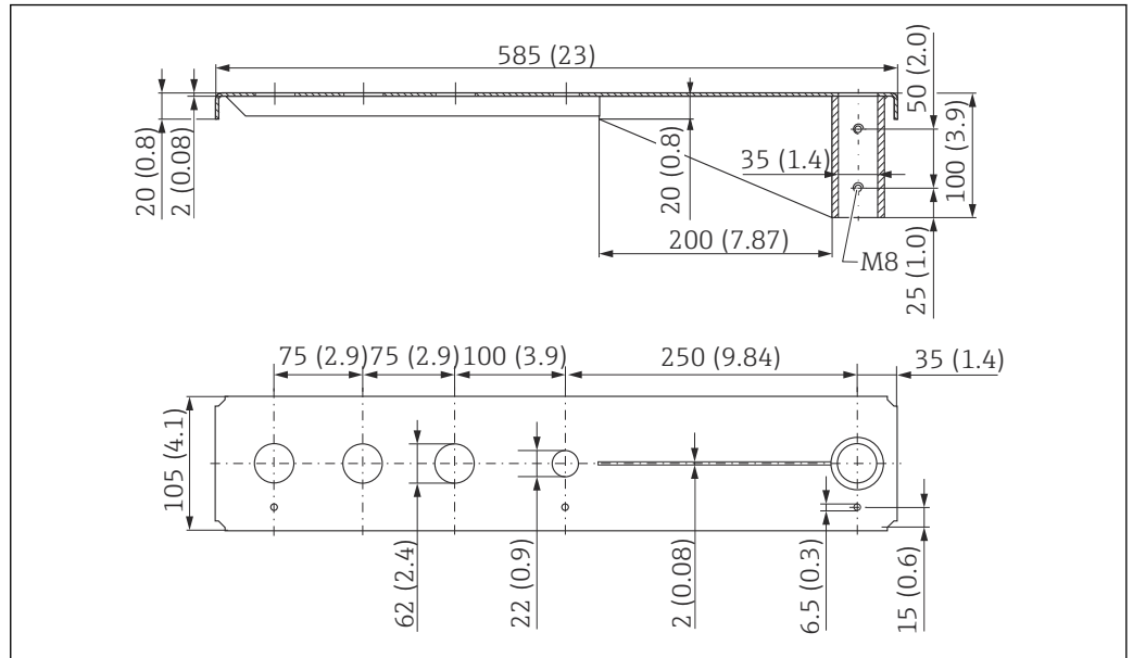
32 Dimensions. Unit of measurement mm (in)
