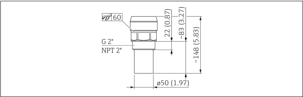
19 Dimensions of sensor. Unit of measurement mm (in)
