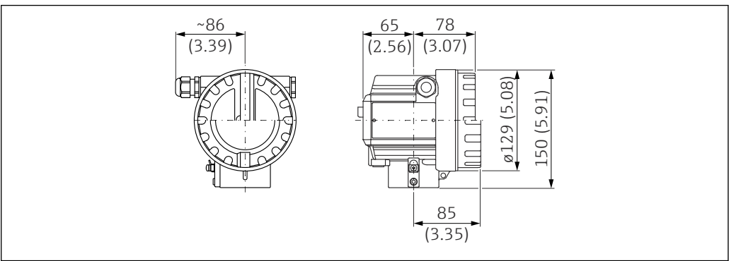
17 Dimensions of F12 housing. Unit of measurement mm (in)
