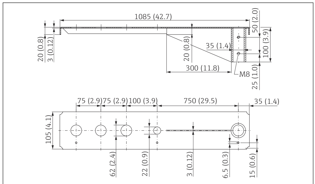
33 Dimensions. Unit of measurement mm (in)
