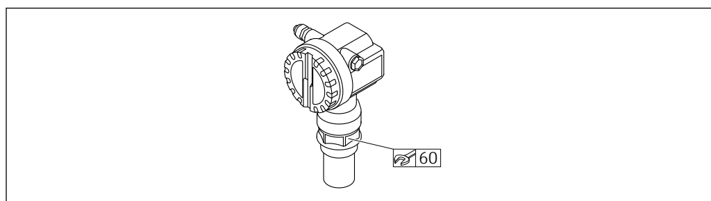
13 Mounting at threaded boss, width across flats AF60
