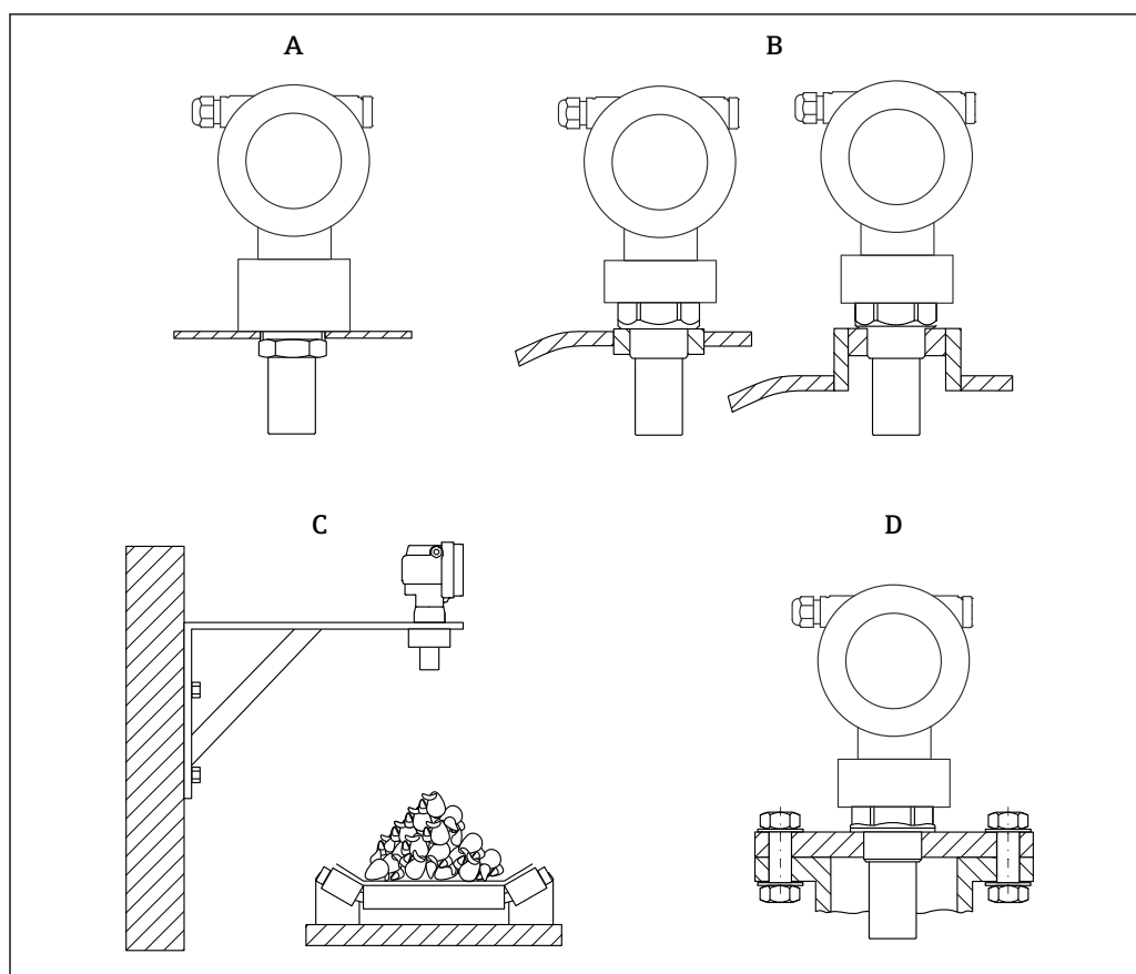
12 Mounting examples
