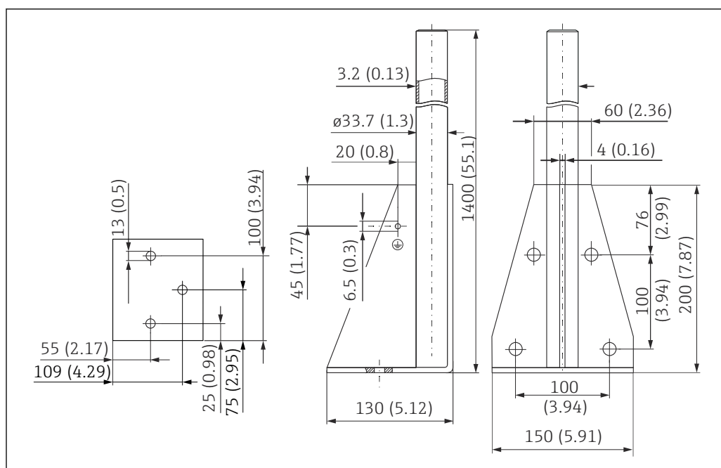
30 Dimensions. Unit of measurement mm (in)
