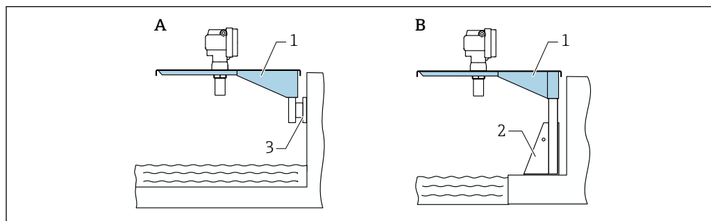
34 Cantilever with mounting stand or wall bracket
