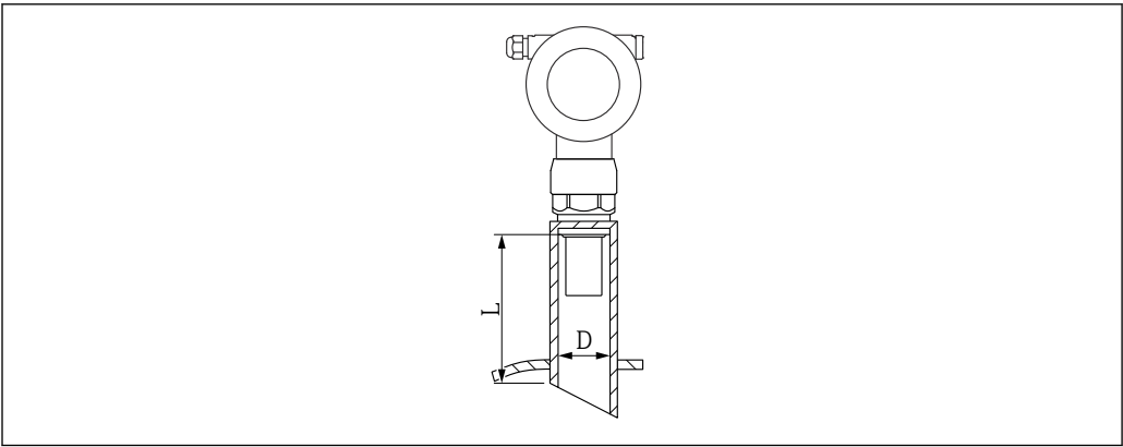
16 Definition of nozzle length L and nozzle diameter D
