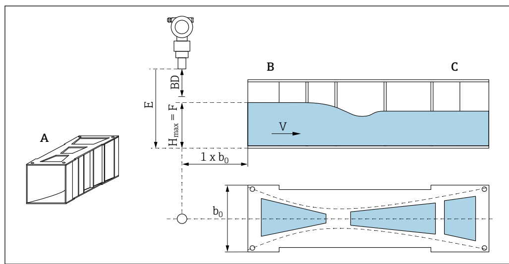
10 Khafagi-Venturi flume (example)
