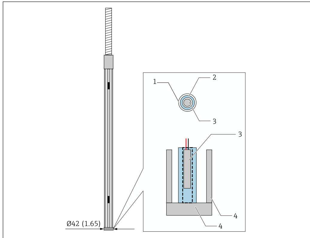
33 WB probe design. Unit of measurement mm (in)
