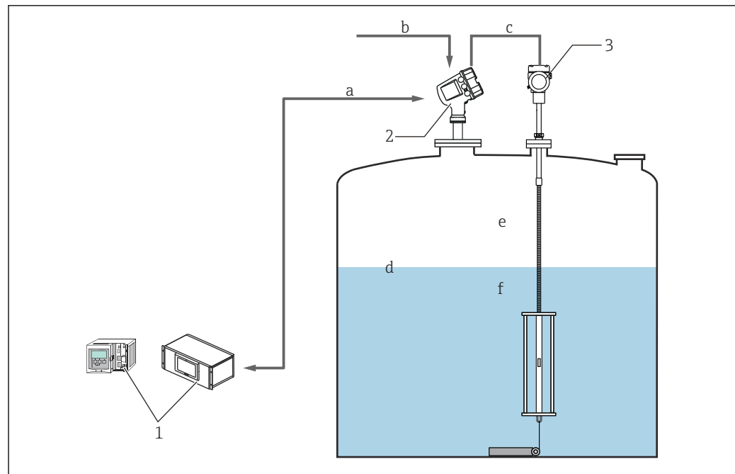
3 NMT81 Ex ia and NMR8x combination
